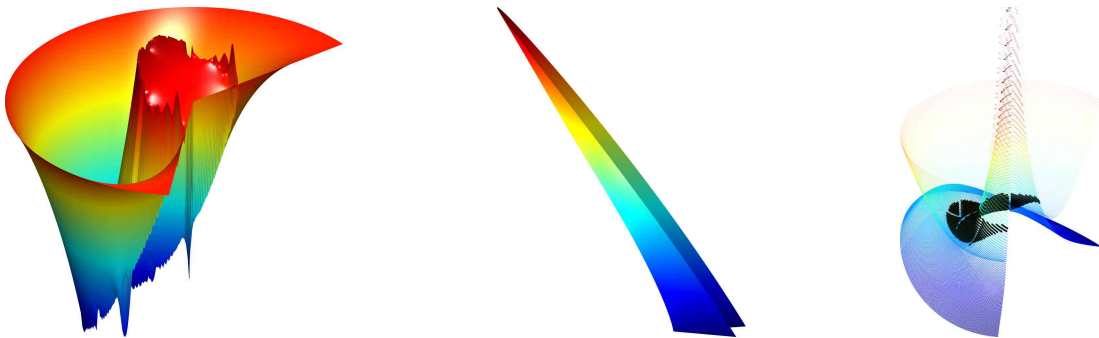
Fig. 5.1. Example 1: u_h (left), y_h (middle), and active set of all T with |\nabla y_h|_T = \psi(x_T) (right) for l = 6 .
